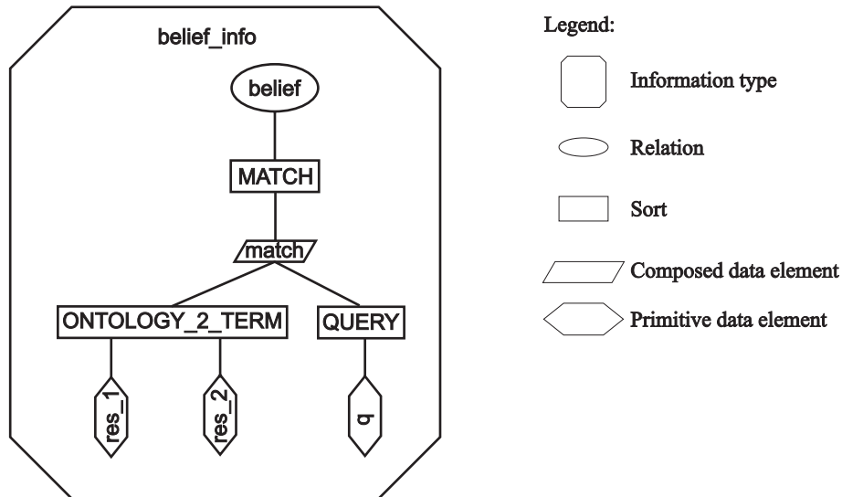
Figure 9.3: Information type for the internal information of the broker agent.
