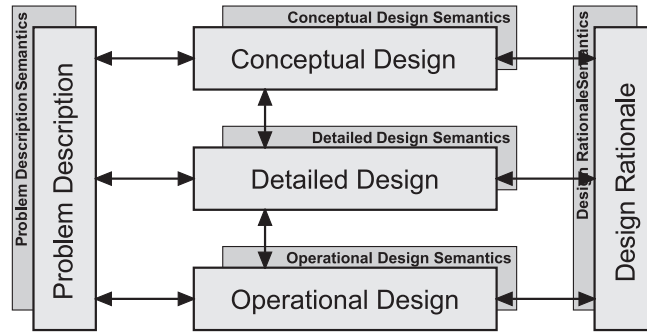
Figure 9.1: The three layers of the DESIRE modelling framework.
