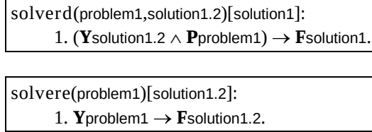
Figure 12.2: Refined Problem Solving Agents (from Fisher & Wooldridge, 1997)
