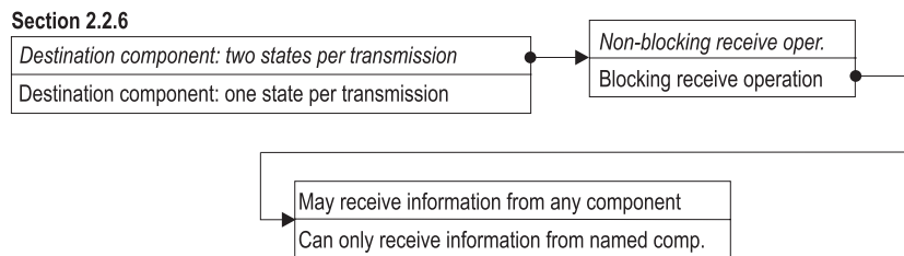
Figure 2.5: Relations between commitments in Section 2.2.6.
